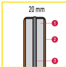
UPHOLSTERED SCREEN WITH FLEXIBLE PROFILE - e=20mm
