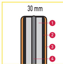
UPHOLSTERED SCREEN WITH FLEXIBLE PROFILE - e=30mm
