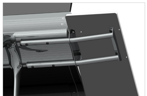
Steel bracket (steel tube \varnothing 25 x 1,5 mm)
