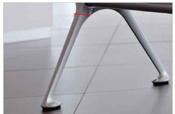
Leg thickness 28 x 34 mm. Solid moulded aluminium
