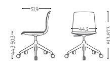
Swivel base with 5-spoke and castors Base de 5 radios con ruedas
