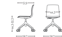
Swivel base with 4-spoke and castors Base de 4 radios con ruedas
