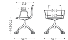
Swivel base with 4-spoke and castors with Closed arms without armrest Base de 4 radios con ruedas con brazo cerrado sin reposabrazos
